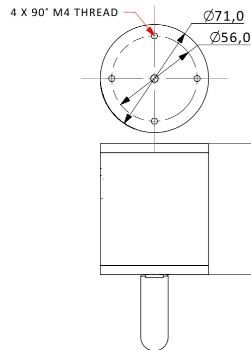
SHAKER BODY
