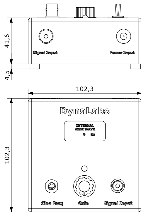
DYNALABS AMPLIFIER
