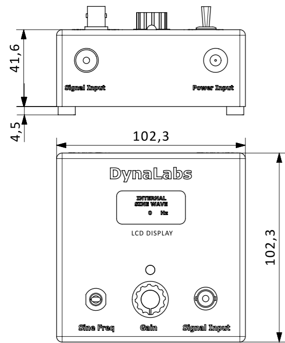
DYNALABS AMPLIFIER
